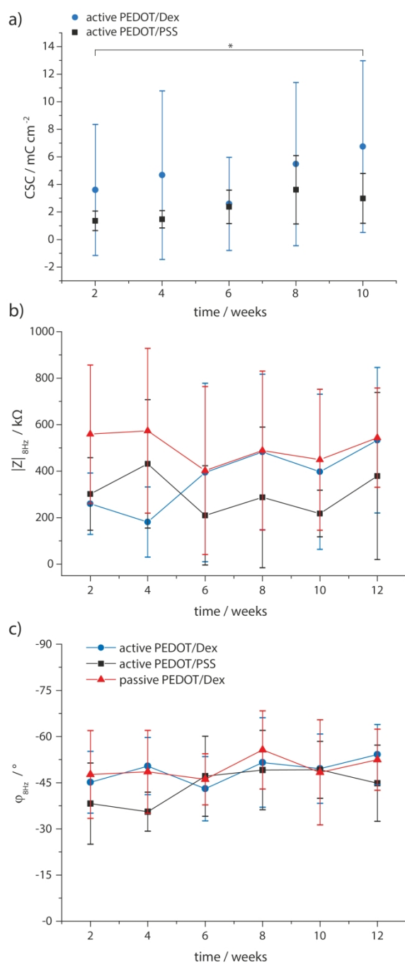
Figure 3: Electrochemical data recorded over 12 weeks in vivo for monitoring of the PEDOT properties. CSC (a), Impedance magnitude (b) and EIS (c) display averaged data for the different animal groups with standard deviation as error bars (n=16). The horizontal line indicates statistical difference for active PEDOT/PSS ( p < 0.01 ).
