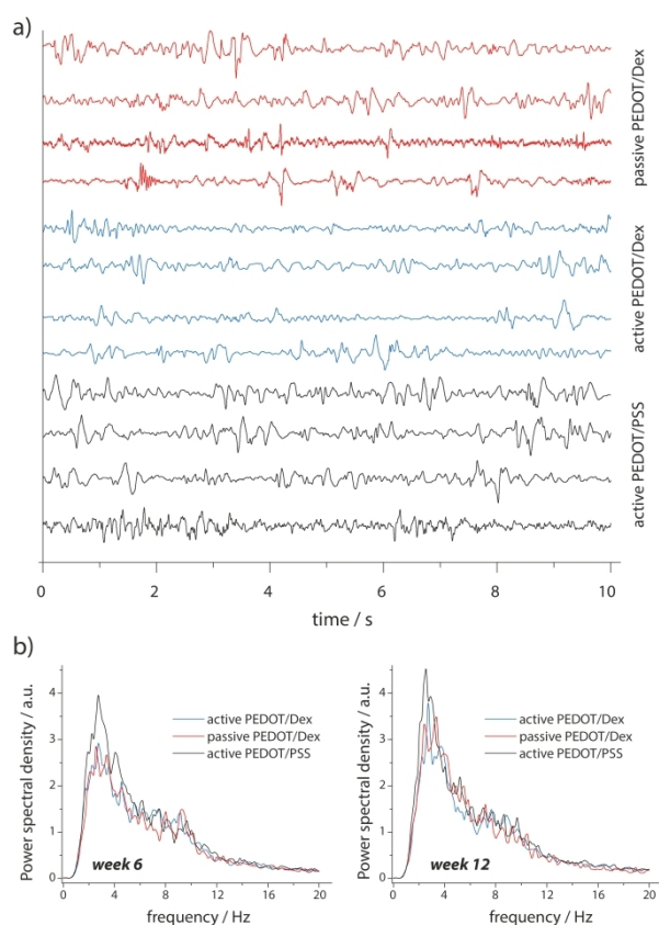
Figure 2: a) Representative LFP data recorded after 12 weeks in vivo from 12 animals demonstrating persistent recording capability for PEDOT/Dex and PEDOT/PSS coated probes. Spectral analysis shows presence of low frequency LFPs over the entire study time (b).
