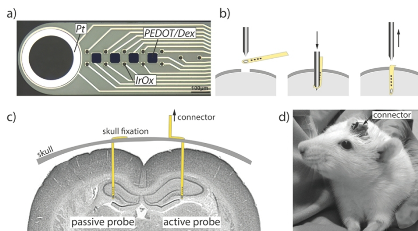
Figure 1: a) Microscope image of a polyimide neural probe with 4 PEDOT/Dex coated electrode sites shown in blue. Probe insertion is performed according to the process shown in b) with an optical fibre as guiding tool. The final placement of the electrodes can be seen in c). Both the passive probe (control) and the active probe (functionalized) are fixated to the skull. The connection of the active probe to the recording / stimulation equipment is achieved via a connector placed on the head of the animal (d).
