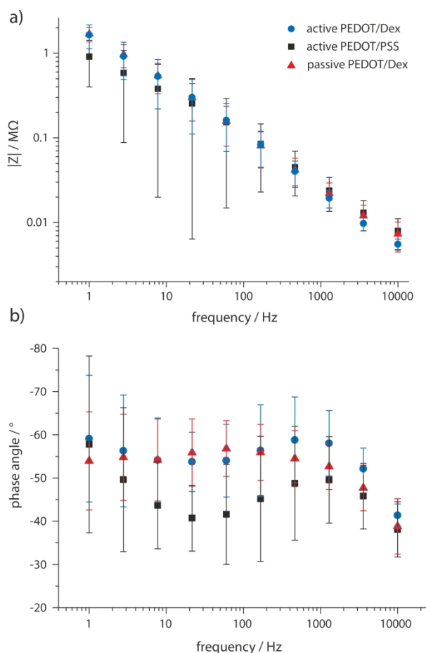
Figure 4: EIS spectrum recorded at week 12 post implantation shows similar characteristics for all animal groups in the impedance magnitude (a) and for the phase angle (b). Error bars denote standard deviation (n=16).
