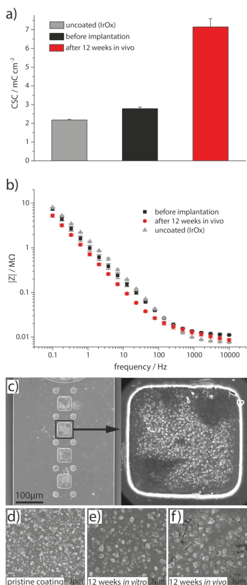
Figure 6: Comparison of CSC (a) and impedance magnitude (b) for a PEDOT/Dex coated probe before implantation and after 12 weeks in vivo . Error bars denote standard deviation ( n=4 ). High resolution SEM shows fully intact PEDOT/Dex coatings after 12 weeks of implantation (c) during which 30 CVs have been applied for drug release. Dark areas in the higher magnification image result from tissue residues after explantation. The morphology of explanted PEDOT/Dex coatings (f) is comparable to PEDOT/Dex films exposed to in vitro stimulation over 12 weeks (e) and shows larger grains in comparison to a pristine polymer film directly imaged after polymerization (d).
